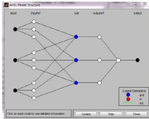
Fig 5: ANFIS structure.
